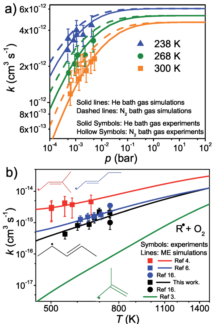
Fig. 4 This figure depicts the \text{CH}_3\text{-CH=CH-CH=CH-CH}_3 + O_2 rate coefficient as a function of temperature and pressure. Below 300 K (a), the rate coefficient describes the \text{CH}_3\text{-CH=CH-CH=CH-CH}_3 + O_2 \rightarrow \text{CH}_3\text{-CH(OO}\cdot\text{)-CH=CH-CH}_3 recombination reaction. Above 500 K (b), the (phenomenological) rate coefficient describes the pressure independent \text{CH}_3\text{-CH=CH-CH=CH-CH}_3 + O_2 \rightarrow bimolecular products reaction.
