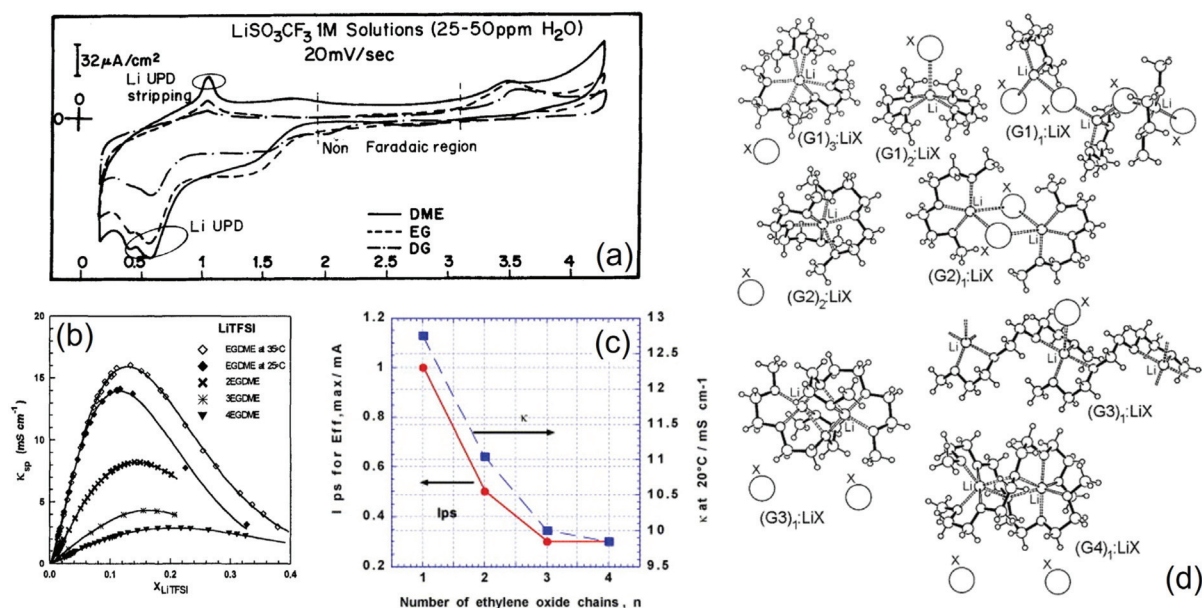
Fig. 2 (a) Typical steady-state voltammograms obtained from polycrystalline gold electrodes in 1 M LiTf solutions of G1 (DME), ethyl glyme (EG) and G2 (DG). Scan rate: 20 mV \text{s}^{-1} . Li underpotential deposition and stripping peaks and the non-Faradaic region are marked. Reproduced with permission. 16 Copyright © 1996 Elsevier Science Ltd. (b) Specific conductivity ( \kappa ) at 25 °C of LiTFSI in glymes, that is, DME (EGDME; \kappa at 35 °C is also shown), G2 (2EGDME), G3 (3EGDME), and G4 (4EGDME). Reproduced with permission. 17 Copyright © 1998 Plenum Publishing Corporation. (c) Relationship between electrolyte conductivity ( \kappa ) and charge–discharge cycling current ( I_{\text{ps}} ) for the maximum value of cycling efficiency of lithium ( \text{Eff}_{\text{max}} ) and n for 1 M \text{LiPF}_6\text{--EM}_{80}/n\text{G}_{20} , where \text{EM}_{100-x}/n\text{G}_x represents the mixed solvent of EC/MEC (3 : 7) and n -glyme (mixing volume ratio = 100 – x : x ), with plating charge ( Q_{\text{p}} ) of 0.025 mA h. Reproduced with permission. 19 Copyright © 2003 Elsevier Ltd. All rights reserved. (d) Schematic illustrations of various glyme–LiX solvate structures with G1, G2, G3, and G4. Reproduced with permission. 21 Copyright © 2006 American Chemical Society.
