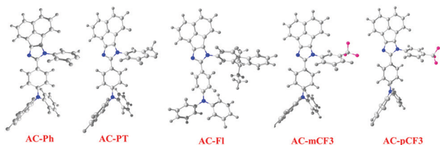
Fig. 4 Optimized geometry of AC-derivatives.
