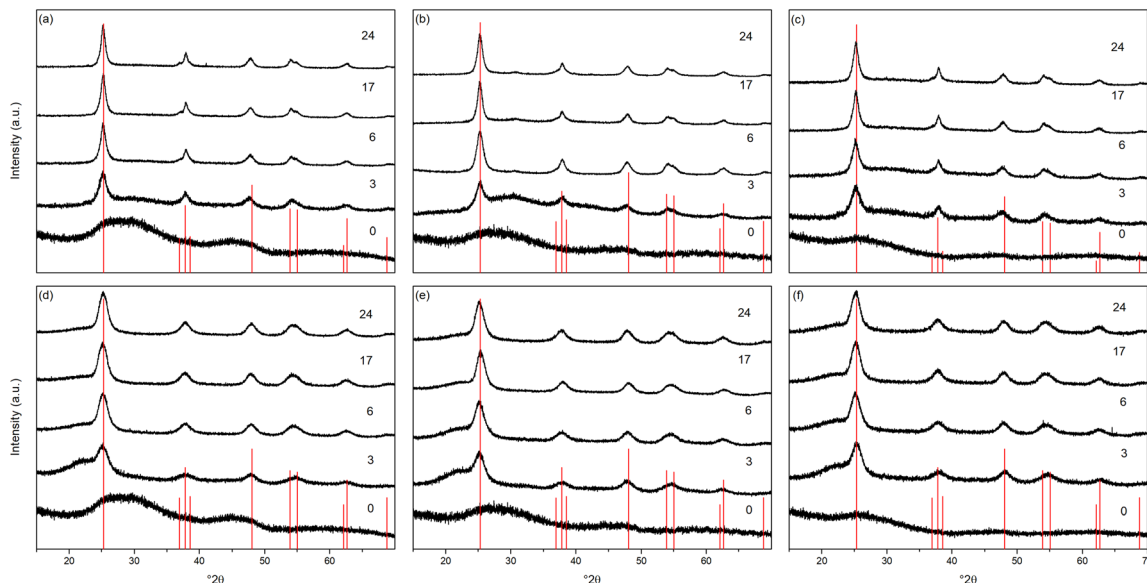
Fig. 4 X-ray diffraction patterns of titania doped with (a) nickel, (b) copper, and (c) cobalt treated hydrothermally at 150 °C for the indicated times and the corresponding (d) nickel, (e) copper, and (f) cobalt doped titania treated solvothermally in trifluoroacetic acid at 150 °C for the indicated times. Data have been normalised and offset for clarity.
