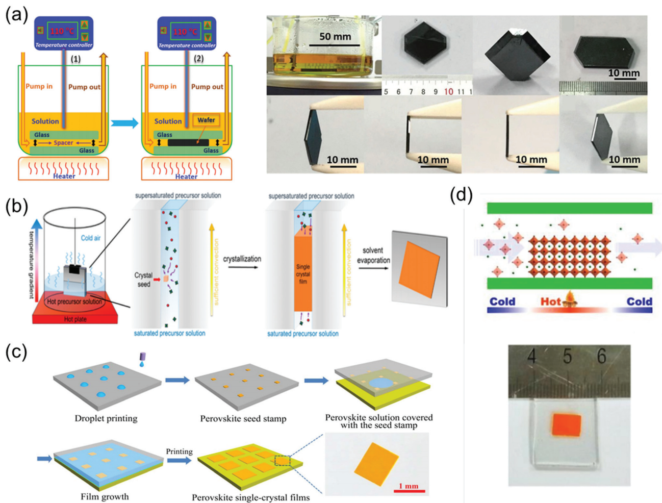
Fig. 9 (a) Schematic illustration of the ultrathin MAPbI 3 single-crystal wafer preparation and photograph of the single-crystal wafer growing in the microreactor system with different thicknesses and shapes. Reproduced with permission. 86 Copyright 2016, Wiley-VCH. (b) Schematic illustration of a spatially confined solution-processed strategy for on-substrate growth of various hybrid perovskite single-crystal thin films. Reproduced with permission. 87 Copyright 2016, RSC. (c) Schematic illustration of the scalable growth of single-crystal perovskite thin-film arrays prepared using the inkjet printing method. Reproduced with permission. 88 Copyright 2018, AAAS. (d) Photograph of an MAPbBr 3 laminar single crystal grown on FTO glass. Reproduced with permission. 89 Copyright 2017, RSC.
