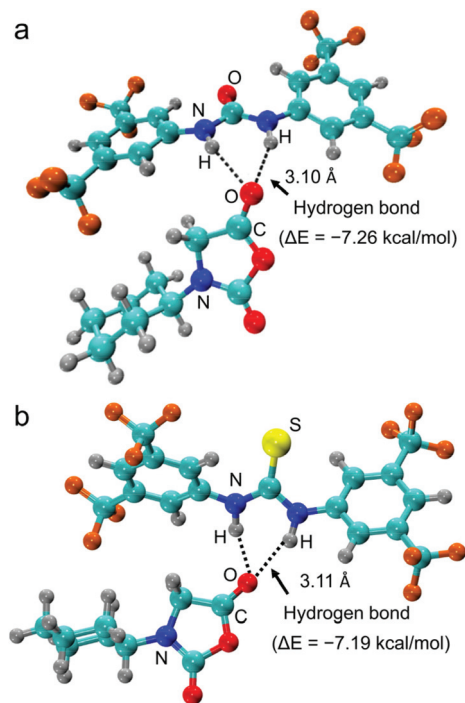
Fig. 5 The DFT-optimized geometry structure showing the hydrogen bonding interaction between (a) U-O and cyclohexyl-NNCA in THF (silver: H, cyan: C, blue: N, red: O, yellow: S and brown: F).
