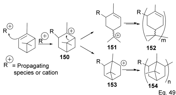
Scheme 43 Cationic polymerization of \delta -pinene mediated by ( \text{SbCl}_3/\text{AlCl}_3 ).
