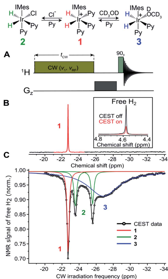
Fig. 12 Upper panel: Molecular diagram of the exchange between the main organometallic complex (SABRE catalyst) [Ir(IMes)(H) 2 (Py) 3 ] + Cl − (1) and its intermediates 2 and 3 in solution (methanol-d 4 ). Lower panel: (A) Experimental 1 H NMR CEST scheme. Continuous wave (CW) irradiation with an amplitude (ν 1 = 50 Hz) is applied for 3 s at a particular offset frequency ν RF and the integral of the free H 2 signal is recorded; then the offset frequency is incremented, and the experiment is repeated again yielding the CEST spectrum. (B) Standard 1 H NMR (500 MHz) spectrum of 1 in methanol-d 4 . The inset shows the CEST effect on the free H 2 resonance when saturation is applied to the hydrides of 1 (ν RF = 22.72 ppm). (C) 1 H NMR CEST spectrum of 1 in methanol at 280 K showing the presence of dihydride intermediates 2 and 3. Black: experimental data; red, blue and green lines are Lorentzian fits (for details see Knecht et al. 180 ).
