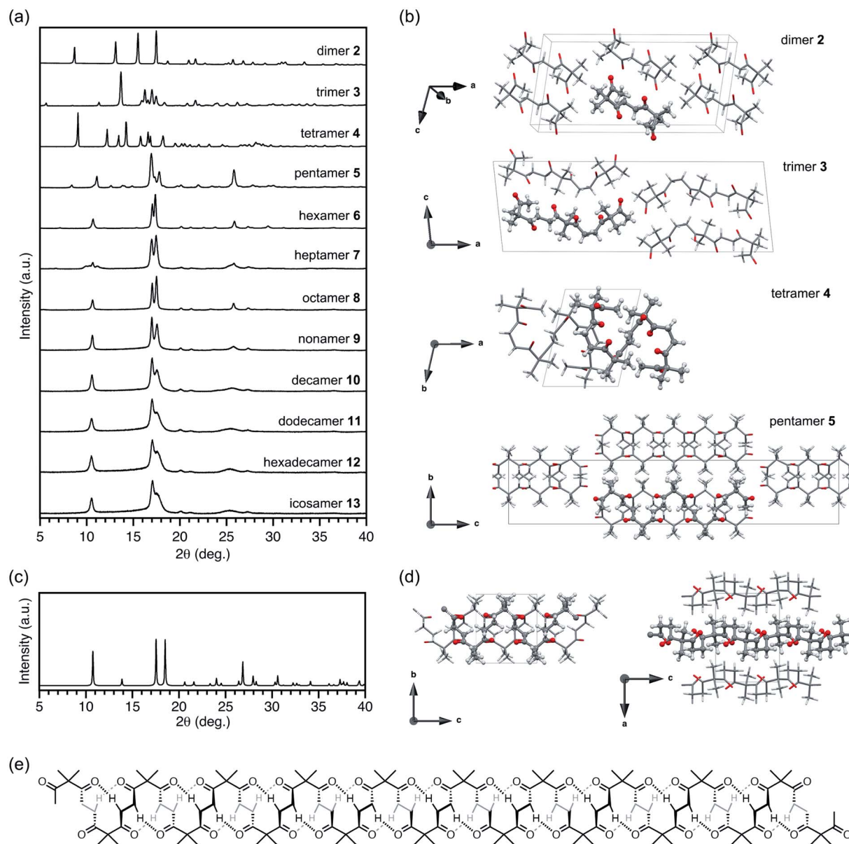
Fig. 2 (a) PXR D patterns of discrete oligomers 2–13. (b) Conformations and packing structures of 2–5 obtained by SCXR D analysis. (c) Simulated PXR D pattern of the energy minimized crystal structure of infinite polyketones. (d) Energy minimized packing structure of infinite polyketone crystals. (e) Chemical structure of icosamer 13 in the helical conformation.
