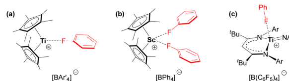
Fig. 7 Fluoroarene complexes of electrophilic transition metals. (a) [(Cp*) 2 Ti( \kappa^1 -FC 6 H 5 )] [BAR' 4 ] (Ar' = Ph or C 6 F 5 ), (b) [(Cp*) 2 Sc( \kappa^1 -FC 6 H 5 ) 2 ] [BPh 4 ], and (c) [(nacnac)Ti=NAr( \kappa^1 -FC 6 H 5 )] [B(C 6 F 5 ) 4 ] (nacnac = {CH(C t Bu)NAr} 2 - ; Ar = 2,6-diisopropylphenyl). 56–58
