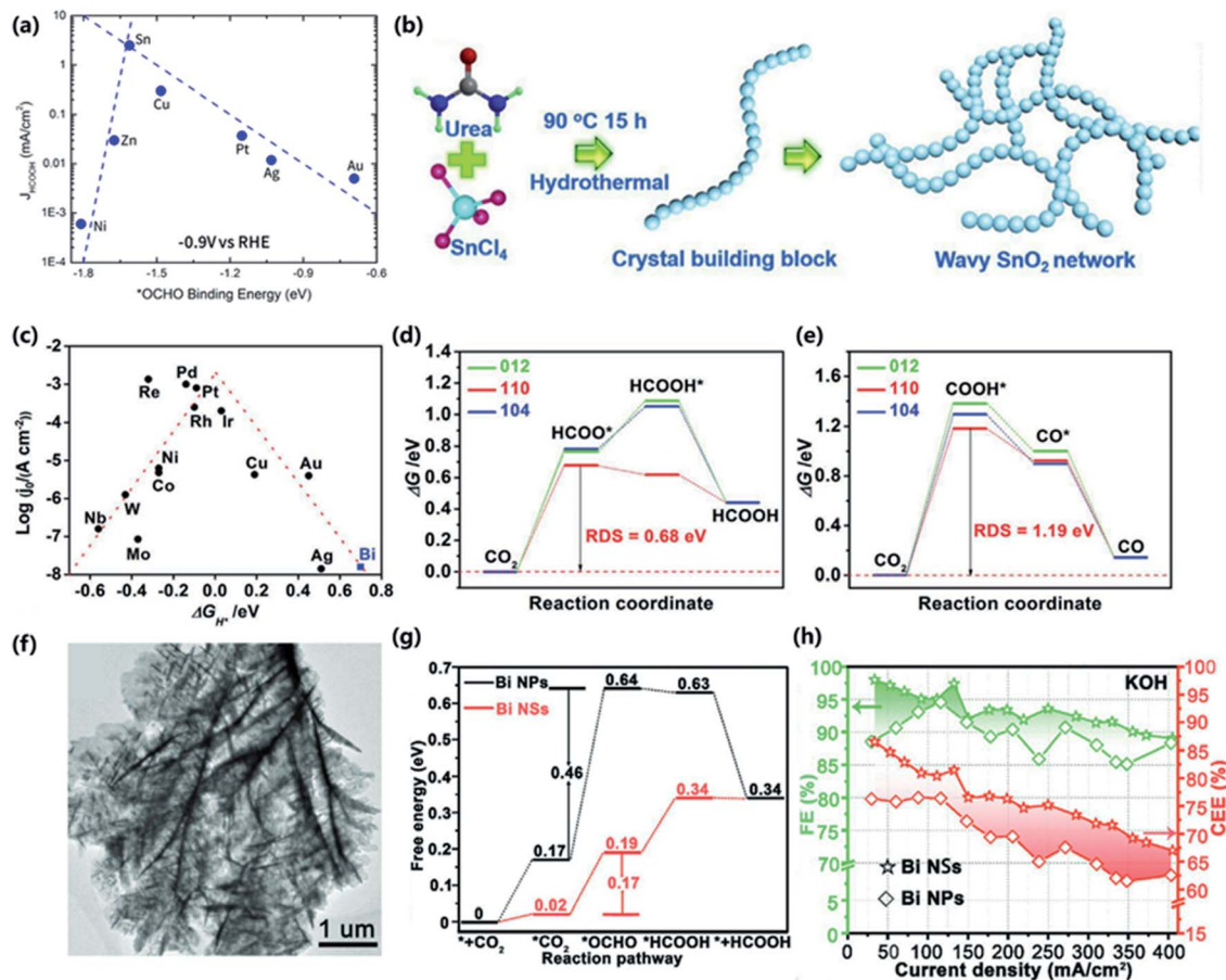
Fig. 4 (a) Volcano plot using ^*\text{OCHO} binding energy as a descriptor for \text{HCOO}^- partial current density at -0.9 V vs. RHE. Adapted with permission. 60 Copyright 2017, the American Chemical Society. (b) Synthetic process towards NW-SnO 2 . Adapted with permission. 65 Copyright 2020, Elsevier. (c) Volcano plots of j_0 as a function of the \Delta G_{\text{H}^+} for Bi and other catalysts. (d) Gibbs free energy diagrams of Bi for the reduction of CO 2 into HCOOH. (e) Gibbs free energy diagrams of Bi for the reduction of CO 2 into CO. Adapted with permission. 67 Copyright 2020, Wiley-VCH. (f) TEM image of Bi NSs. (g) Gibbs free energy profiles for CO 2 electroreduction to HCOOH on Bi NPs and Bi NSs. (h) FEs and CEEs of formic acid over two electrocatalysts in 1 M KOH. Adapted with permission. 68 Copyright 2020, Wiley-VCH.
