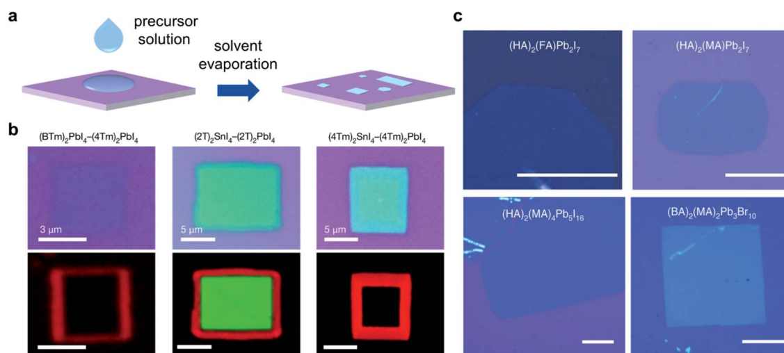
Fig. 5 Synthesis and morphology of perovskite nanosheets. (a) Schematic illustration of direct synthesis of 2D halide perovskite thin sheets. (b) Optical and PL images of (\text{BTm})_2\text{PbI}_4-(4\text{Tm})_2\text{PbI}_4 , (2\text{T})_2\text{SnI}_4-(2\text{T})_2\text{PbI}_4 and (4\text{Tm})_2\text{SnI}_4-(4\text{Tm})_2\text{PbI}_4 heterostructures 79 (Copyright: 2020, Nature). (c) Optical images of \text{HA}_2\text{FAPb}_2\text{I}_7 , \text{HA}_2\text{MAPb}_2\text{I}_7 , \text{HA}_2\text{MA}_4\text{Pb}_5\text{I}_{16} and \text{BA}_2\text{MA}_2\text{Pb}_3\text{Br}_{10} nanosheets (scale bars: 25\ \mu\text{m} ) 80 (Copyright: 2021, Nature Nanotechnology).
