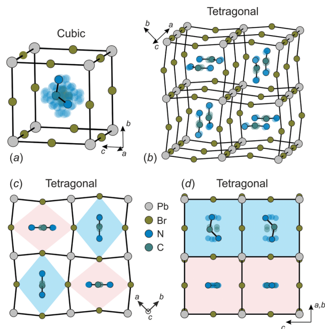
Fig. 1 Structure of FAPbBr 3 in the (a) cubic and (b–d) tetragonal phases. There are 48 and 4 equivalent orientations (indicated by transparent atoms) of FA cation in the cubic and tetragonal phase, respectively. Color coding in (d) corresponds to the colors of the rhombic channels in (c). Structural data taken from ref. 27.
