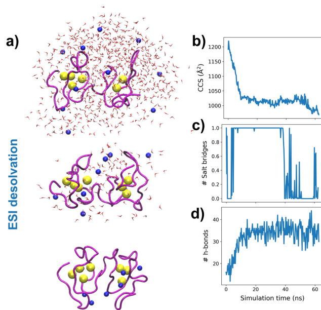
Fig. 3 Molecular dynamics simulations. Snapshots of the desolvation process at different simulation times for an aqueous nanodroplet containing Zn 7 MT2 and Na + as a charge carrier (a) and analysis of CCS (b), salt-bridges (c) and h-bonds (d) as a function of desolvation time. Yellow and blue spheres represent Zn 2+ and Na + , respectively, and the solvent molecule oxygen atoms are shown in red. The protein backbone is shown in magenta.
