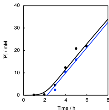
Fig. 7 Time courses of the product formation in the O_2/1/PhCHO system (black line) and that of the reaction where 1 was added after 2 h (blue line). Reaction conditions: [PhCHO] = 0.2\text{ M} , [cyclohexane] = 2.0\text{ M} , [1]_0 = 0.025\text{ mM} at 40\text{ }^\circ\text{C} under O_2 .
