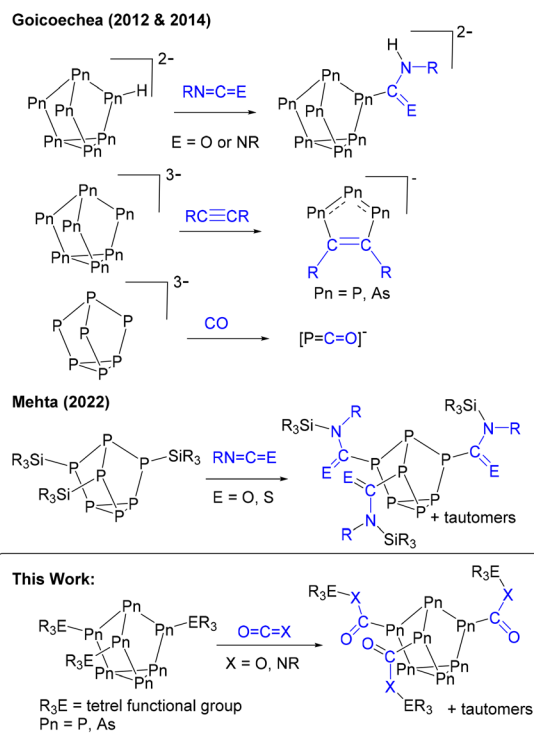
Fig. 1 Previously reported reactions of [Pn_7] clusters with small molecules and this work.
