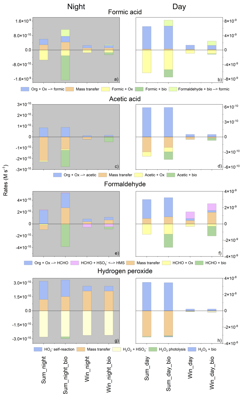
Fig. 4 Aqueous chemical budgets for formic and acetic acids, formaldehyde and H_2O_2 during summer and winter simulations at day and night, with or without biodegradation. Production rates (positive values) and destruction rates (negative values) were integrated over the entire simulation (the first 10 minutes were excluded in these calculations). Chemical (blue) and biological (light green) sources are presented together with the chemical (yellow) and biological (green) sinks. The equilibrium for the formaldehyde budget is marked in pink. Mass transfer is presented in orange. Ox: oxidants; "Org + Ox": a sum of organic compounds reacting with oxidants; " H_2O_2 self-reaction": reaction of H_2O_2^*/O_2^* with itself; HMS: hydroxymethanesulfonate. Note that the scale for the rates is different for simulations at day and night.
