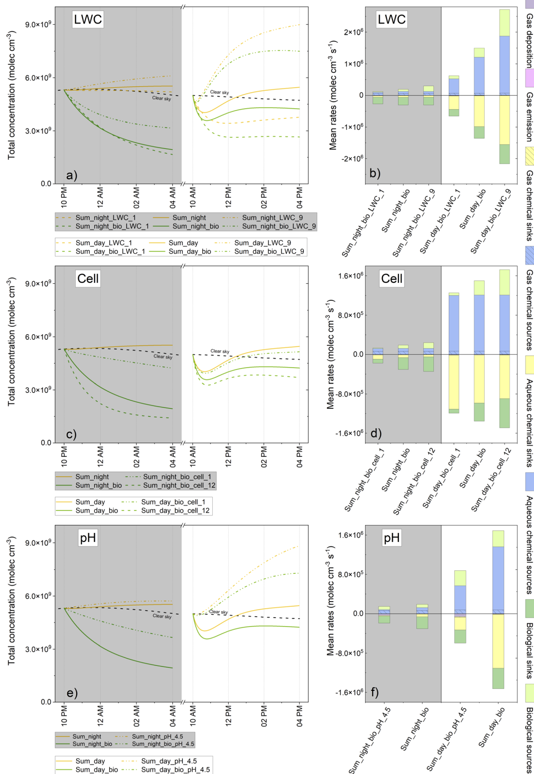
Fig. 7 Total concentrations (left) and multiphase chemical budgets (right) for formic acid when considering the LWC (“_LWC_1”: 1 \times 10^{-7} v/v; “_LWC_9”: 9 \times 10^{-7} v/v), the cell concentration (“_cell_1”: 1.27 \times 10^4 cells mL -1 ; “_cell_12”: 12.35 \times 10^4 cells mL -1 ) and the pH variations (“_pH_4.5”: 4.5). The total concentration is the sum (in molecules cm -3 ) of the aqueous and the gas phase concentrations of the different simulations with (green) and without (yellow) biodegradation. The total chemical budget considers the aqueous transformations: chemical sinks (hatched yellow) and sources (hatched blue) as well as the emission (pink) and deposition (purple) processes. The mass transfer was zero as it balanced between the gas and the aqueous phases.
