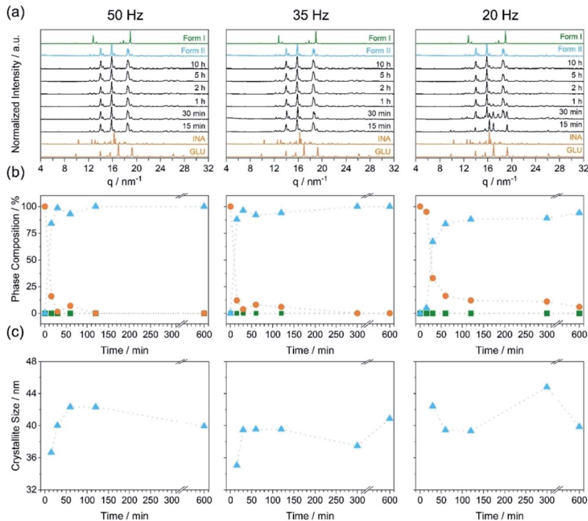
Fig. 3 Results of the milling experiments at ambient temperature of the cocrystal INA:GLU for 50 Hz (left), 35 Hz (middle) and 20 Hz (right) with a milling ball size of 10 mm. (a) PXR D pattern with the diffraction patterns of the starting materials (orange) and Form I (green) and Form II (blue) are given below and above. (b) Phase composition of the milling experiments (sum of INA and GLU (orange circle), Form I (green square) and Form II (blue triangle)). (c) Evolution of the crystallite size of Form II (blue triangle).
