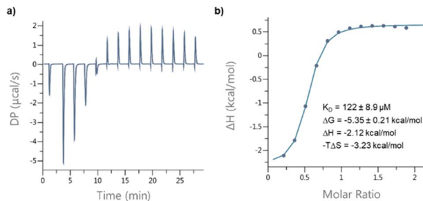
Fig. 7 ITC analysis of the interaction between I and T_{11} in CH_3OH : (a) raw data; (b) fitted curve.
