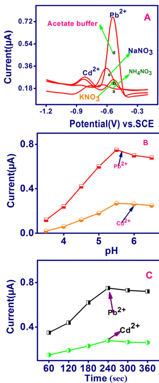
Fig. 4 Effect of (A) supporting electrolyte, (B) pH and (C) preconcentration time on the anodic stripping peak currents of \text{Pb}^{2+} and \text{Cd}^{2+} (8 ppb each) to evaluate TSAB/MWCNT sensor performance in 0.1 M ABS (pH 5.5).
