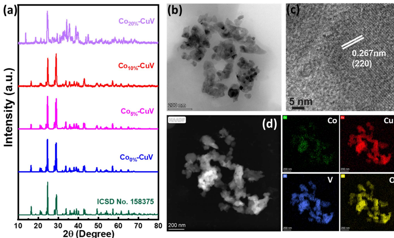
Fig. 1 (a) Powder XRD patterns of \text{CuV} and \text{Co}_{x\%}\text{-CuV} ; (b) TEM image of \text{Co}_{10\%}\text{-CuV} ; (c) HR-TEM image of \text{Co}_{10\%}\text{-CuV} ; (d) HAADF image and elemental mapping of \text{Co}_{10\%}\text{-CuV} obtained at 550 °C under an inert atmosphere.
