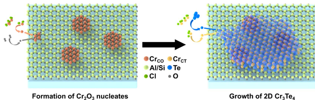
Fig. 4 A schematic diagram illustrating the proposed crystal growth model for epitaxially grown 2D Cr 3 Te 4 on the mica substrate. The process has two steps, with the first step being the formation of Cr 2 O 3 seed particles, and the second step being the growth of Cr 3 Te 4 based on Cr 2 O 3 /Cr 3 Te 4 interfaces.
