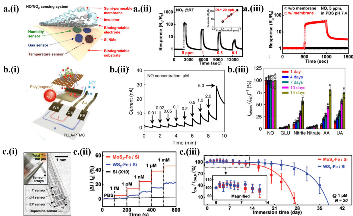
Fig. 5 Transient electronics to monitor NO x and dopamine. (a) (i) The design of NO x gas integrated with temperature and humidity sensors. (ii) The linear dynamic response to various NO 2 concentrations at room temperature with a linear fit to show the estimation of the limit of detection of 20 ppb. (iii) The dynamic response of the gas sensor with and without semipermeable to NO in the PBS solution. This figure has been reproduced under the terms of the Creative Commons Attribution 4.0 International License. 4 Copyright 2020, Springer Nature. (b) (i) The design of the electrochemical NO sensor with Au nanomembrane electrodes on PLLA-PTMC. (ii) The dynamic electrochemical response of the sensor to varying NO concentrations (bias voltage of 0.8 V). (iii) Stability of the NO sensor selectivity showing a decrease after 7 days. This figure has been reproduced under the terms of the Creative Commons Attribution 4.0 International License. 2 Copyright 2020, Springer Nature. (c) (i) Integration of a dopamine sensor with electrophysiology, temperature, and pH sensors in a neural probe. (ii) The relative current change of the neurochemical sensor to various dopamine concentrations. (iii) Change of response to 1 pM dopamine in a buffer solution for 5 weeks. This figure has been reproduced from ref. 5 with permission from John Wiley and Sons, copyright 2022.
