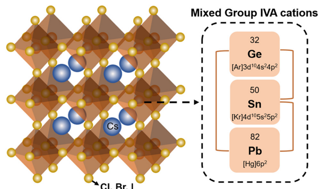
Fig. 1 Crystal structure of the all-inorganic ABX 3 perovskite based on mixed group IVA cations.
