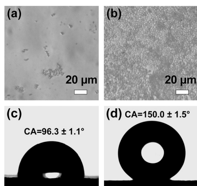
Fig. 5 Optical microscopy images of the top suspension (both pipetting 20 \mu\text{L} of the light irradiation group at (a) 0 min and (b) 20 min (corresponding to Fig. 4b1 and b2, respectively). Water contact angles of (c) pure ZIF-8 and (d) PPy/ZIF-8 micromotors.
