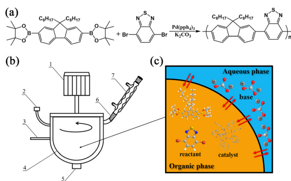
Fig. 1 (a) Reaction scheme of the synthesis of F8BT via the Suzuki cross-coupling reaction. (b) Inner circulation RPB reactor with the following components: 1, rotor; 2, injection inlet; 3, N 2 inlet; 4, thermostatic bath; 5, discharge hole; 6, feed inlet; and 7, condenser. (c) Schematic diagram of the reaction at the interface between organic phase and aqueous phase of the tiny reaction unit of droplet.
