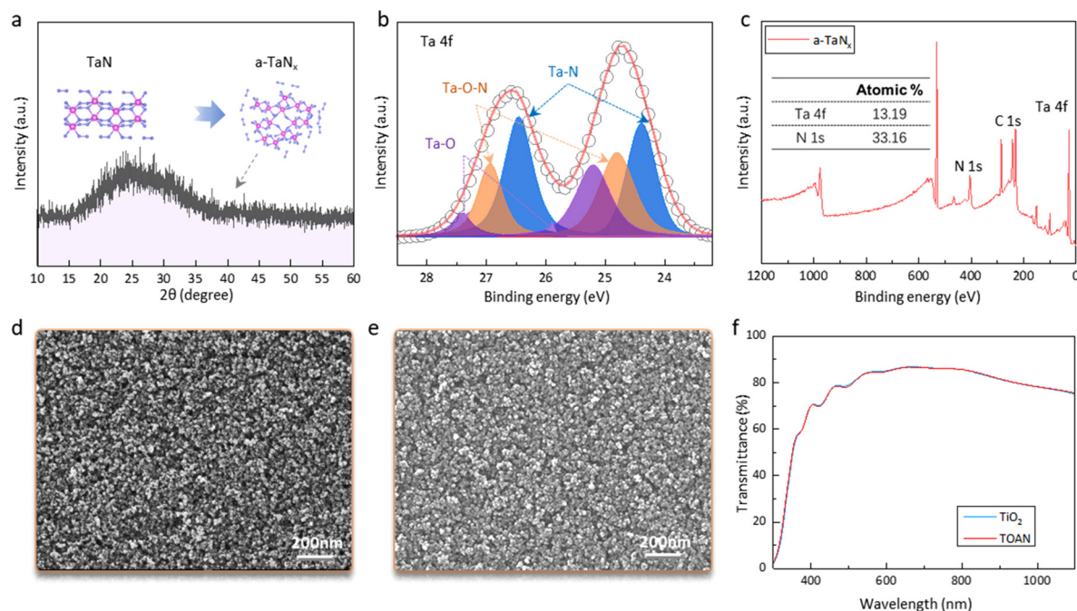
Fig. 1 Construction and characterization of the TOAN ETL. (a) XRD pattern of the ~80 nm a-Ta x film deposited on glass. XPS patterns of (b) Ta 4f and (c) a-Ta x films. The SEM images of (d) TiO 2 and (e) TOAN layers on FTO substrates. (f) The optical transmittance of the TiO 2 and TOAN layers.
