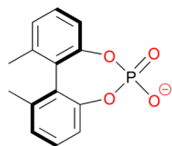
(R)-86
