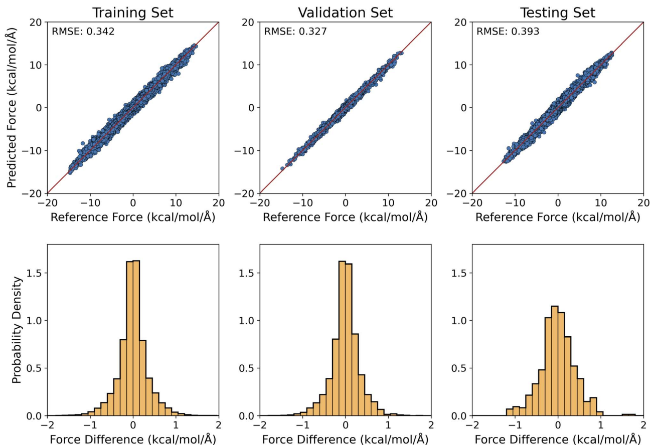
Fig. 3 ML predicted solvation forces acquired from ASEC simulation using trajectory configurations. Top: ML-predicted solvation forces versus reference values (in kcal mol -1 Å -1 ) for the training, validation, and testing sets, which consist of 1245, 51, and 500 configurations, respectively. Bottom: the distribution of errors in the ML-predicted forces.
