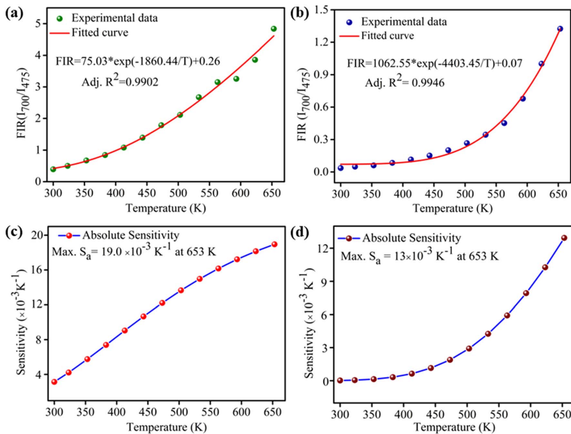
Fig. 6 Exponential fitting of FIR data of non-thermally coupled levels ( ^3F_3 and ^1G_4 ) as a function of temperature for (a) Tm^{3+}/Yb^{3+} : LaVO_4 (b) Tm^{3+}/Yb^{3+} : GdVO_4 phosphors; absolute sensitivity as a function of temperature for (c) Tm^{3+}/Yb^{3+} : LaVO_4 (d) Tm^{3+}/Yb^{3+} : GdVO_4 phosphors.
