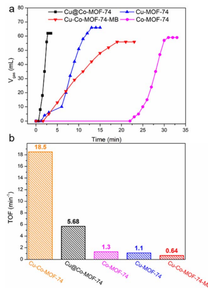
Fig. 4 (a) Gas evolution from aqueous AB and (b) the corresponding TOF values using control samples (25 °C, initial weight of MOF is 50 mg, n AB = 1 mmol).
