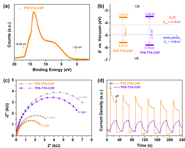
Fig. 4 (a) UPS of the PTZ-TTA-COF. Band structures (b), EIS Nyquist plots (c) and transient photocurrent response (d) of the PTZ-TTA-COF and TPA-TTA-COF.
