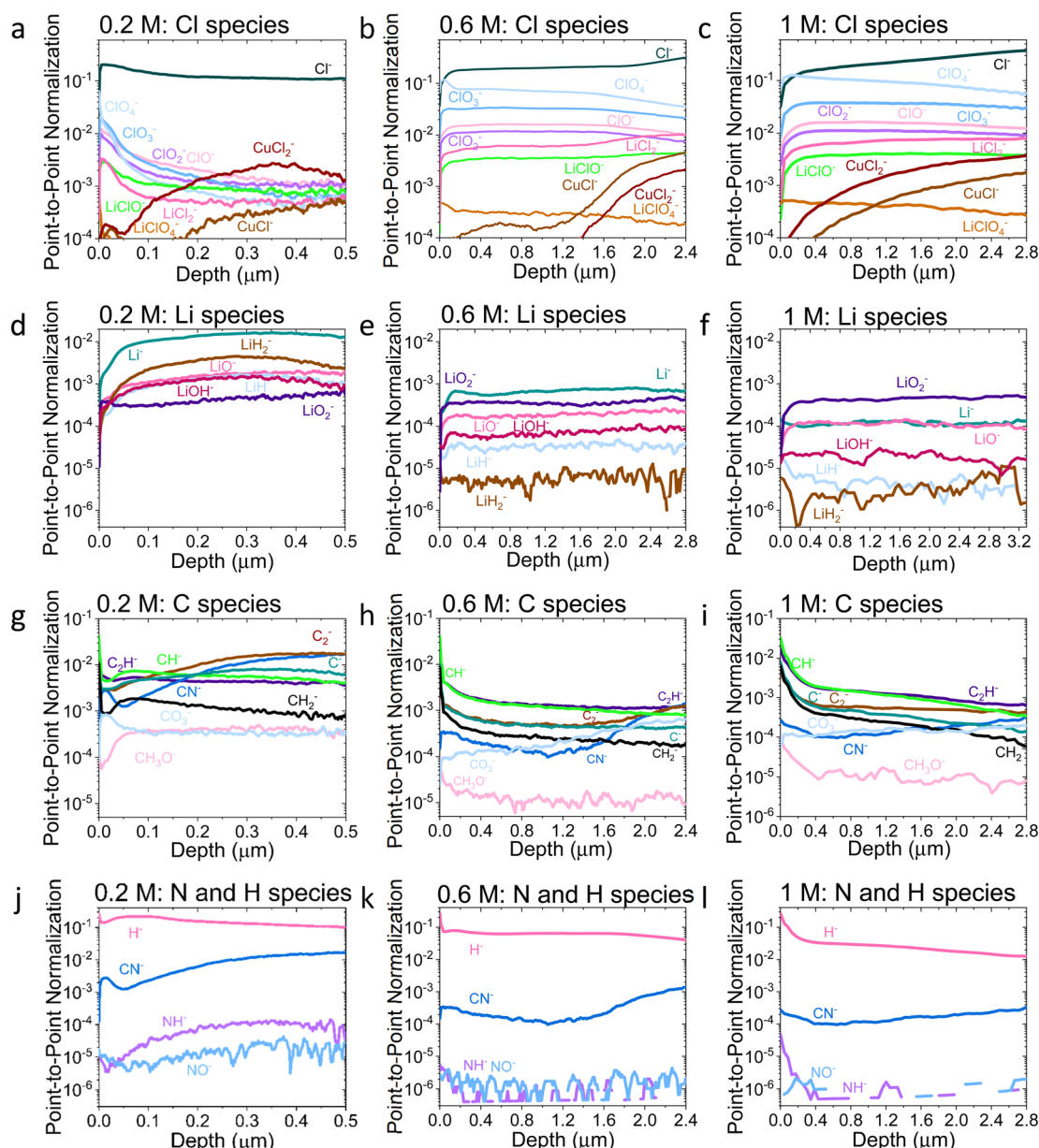
Fig. 3 Comparison of the ToF-SIMS traces for the 0.2 M, 0.6 M, and 1 M LiClO 4 samples on a Cu working electrode after passing -10C under N 2 at -2 mA cm -2 . (a–c) Cl species for 0.2, 0.6, and 1 M samples, (d–f) Li species for 0.2, 0.6, and 1 M samples, (g–i) C species for 0.2, 0.6, and 1 M samples and (j–l) N and H species for 0.2, 0.6, and 1 M samples. All traces normalised to total counts point-to-point. The traces are shown from the surface of the SEI (0 μm) to the Cu surface of that sample. Sputtering was done with Ar + clusters ( n = 1159). Depth is estimated using the crater depth and assuming a constant sputter rate. Crater depth was measured using an optical interferometer. Full experimental details can be found in the ESI section 4b.†
