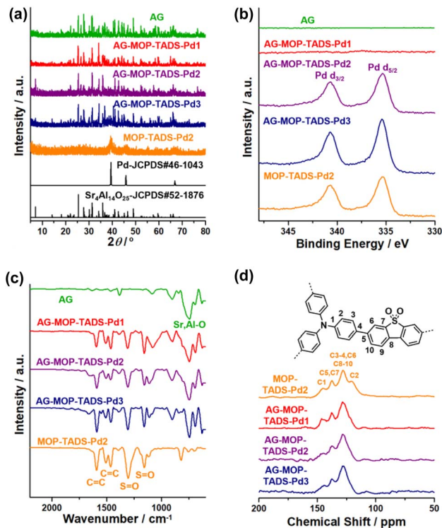
Fig. 4 (a) PXRD patterns, (b) XPS, and (c) IR spectra of AG, AG-MOP-TADS-Pds, and MOP-TADS-Pd2, and (d) solid state ^{13}\text{C} NMR spectra of AG-MOP-TADS-Pds and MOP-TADS-Pd2.
