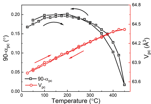
Fig. 2 Temperature dependence of rhombohedral lattice distortion and pseudo-cubic cell volume of 0.7BiFeO 3 -0.3Ba(Ti 0.995 Nb 0.005 )O 3 ceramics.
