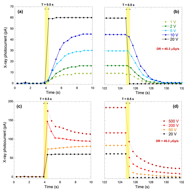
Fig. 8 Rising (a)–(c) and decaying (b)–(d) dynamics of photocurrent pulses recorded during a single “X-ray on” period (120 s) at low (a), (b) and high (c), (d) bias voltages. Dose rate was set to 45.3 \mu\text{Gy s}^{-1} , but similar results have been obtained at all other investigated dose rate values.
