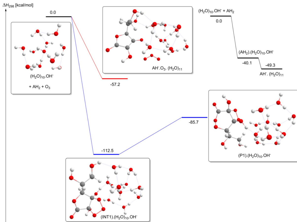
Fig. 8 Enthalpies ( \Delta H_{298} , kcal mol ^{-1} ) calculated for the reactions between ascorbic acid and O_3 on the [(H_2O)_{10} \cdot OH^-] surface.
