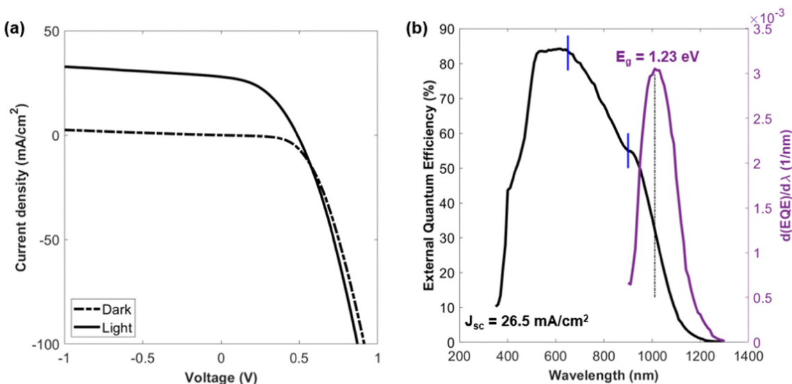
Fig. 4 (a) Champion cell IV curves in the dark (dashed line) and under AM1.5G illumination (solid line). (b) EQE response of the champion CZTGSe cell at 0 V, in black solid line (left vertical axis), and its derivative with respect to wavelength in the purple solid line (right vertical axis). The J_{sc} and E_g values, respectively, extrapolated from the AM1.5G spectral integration and the EQE derivative peak position, are indicated. The dashed black line and blue solid lines are a guide to the eye, respectively, highlighting the peak position of d(EQE)/d\lambda and the hindered carrier collection within the absorber.
