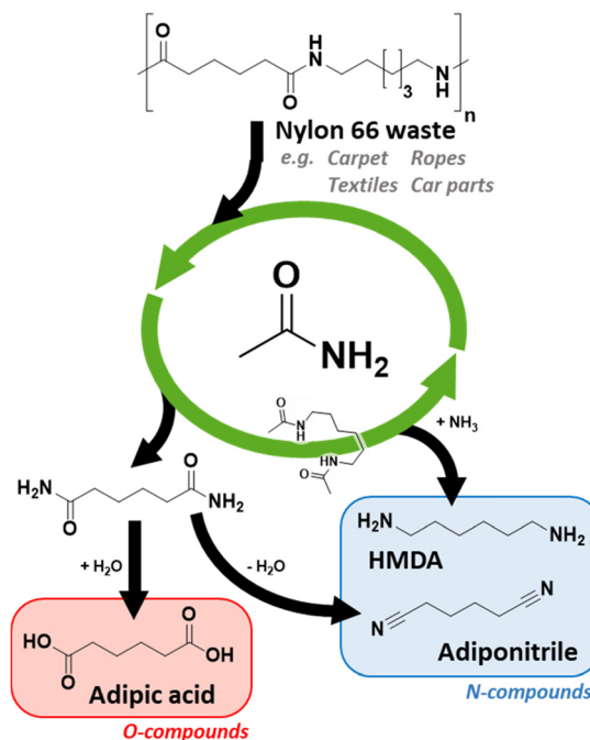
Scheme 2 Complete recycling of Nylon 66 waste based on a transamidation depolymerization technique.
