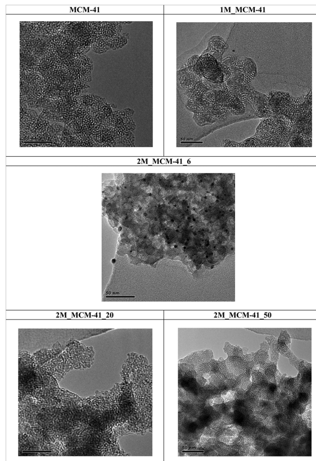
Fig. 11 TEM micrographs of MCM41 and M_MCM41 samples.
