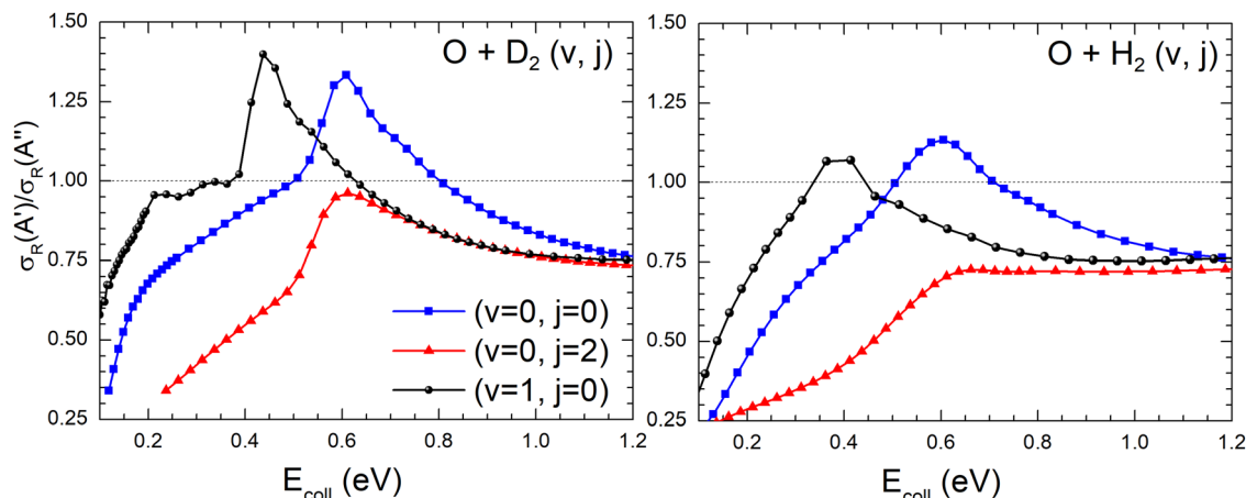
Fig. 9 Comparison of the ratios of the QM cross sections on the {}^3A' and {}^3A'' PES as a function of E_{\text{coll}} for the O({}^3P) + D_2(v,j) (left panel) and O({}^3P) + H_2(v,j) reactions (right panel).
