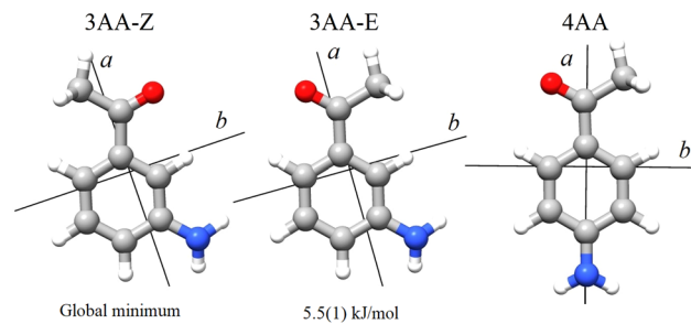
Fig. 2 Principal axis system of 3' and 4'-aminoacetophenone.
