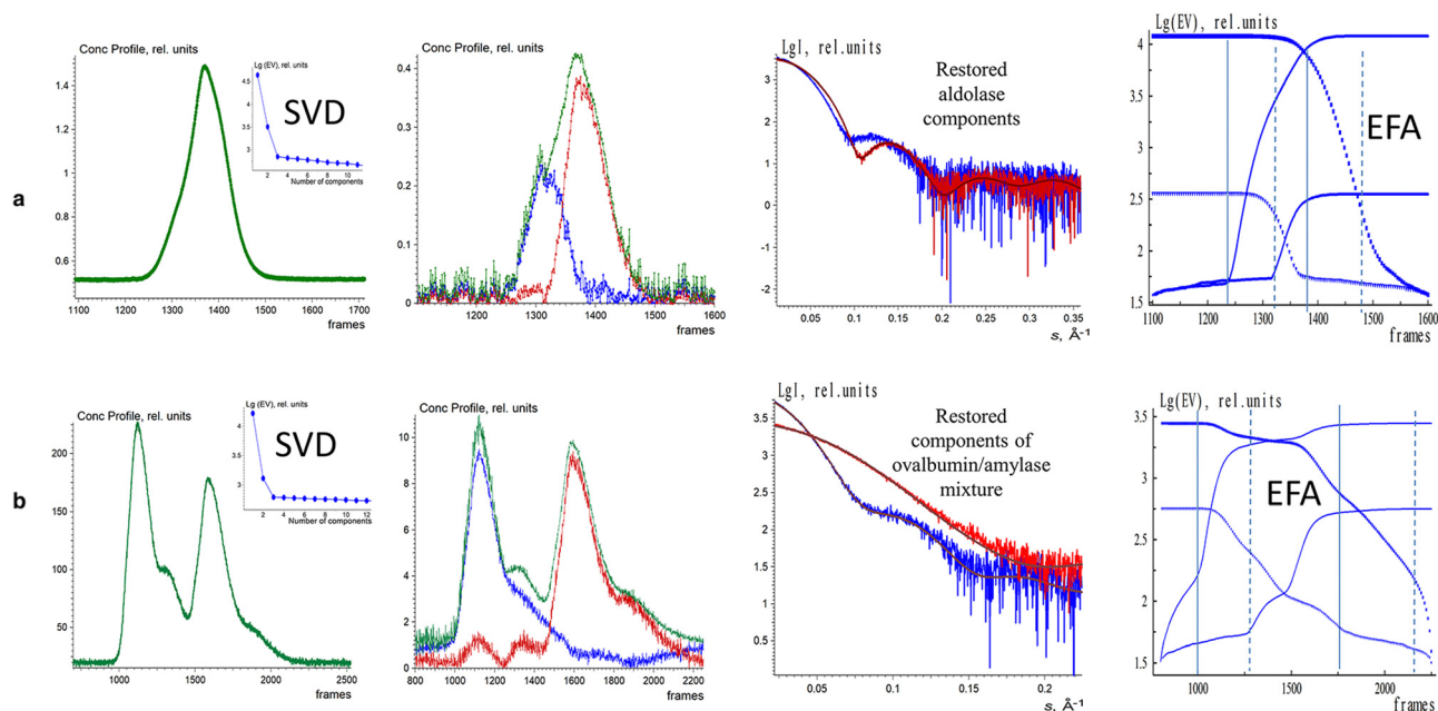
Fig. 3 EFAMIX decomposition of experimental SEC-SAXS data from 2-component systems: aldalase (a) and ovalbumin with beta-amylase (b). In these systems, the first column displays the elution profiles of SEC-SAXS data obtained by CHROMIXS (green) and the SVD of the background corrected SEC-SAXS data. The second column displays the concentration profiles of the components (blue and red curves), and the green curve is the overall concentration profile. The third column displays the EFAMIX restorations and the corresponding fits. The fourth column displays the forward EFA (solid lines) and the backward EFA (circles) plots. Reproduced from Konarev et al. , Protein Sci. , 2022, 31 , 269–282 published by Wiley Periodicals LLC on behalf of The Protein Society under the terms of the Creative Commons Attribution Non-Commercial License https://creativecommons.org/licenses/by-nc/4.0/ .
