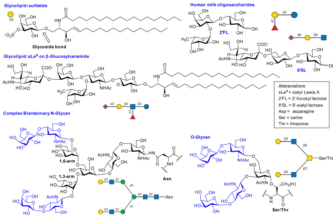
Fig. 2 Selected examples of lectin ligands. SNFG nomenclature was generated using glyco-glyph. 8 The N -glycan and O -glycans shown are bivalent glyco-clusters where two LacNAc disaccharides (blue) are presented on saccharide scaffolds (black).
