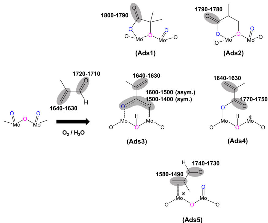
Fig. 3 Proposed ring surface species under MAL reaction conditions at 320 °C over HPA catalysts: 5-membered ring lactone-type species ( Ads1 ), 6-membered ring lactone-type species ( Ads2 ), bidentate methacrylate species ( Ads3 ), monodentate methacrylate species ( Ads4 ), and \pi -adsorbed species [ Ads5 ].
