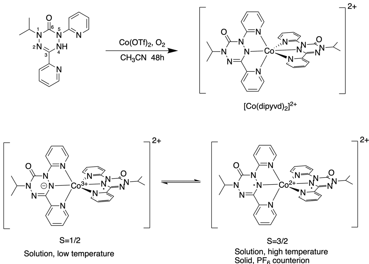
Scheme 1 Synthesis of [Co(dipyvd) 2 ] 2+ showing ligand numbering scheme (top) and the [Co(dipyvd) 2 ] 2+ valence tautomeric equilibrium (bottom).
