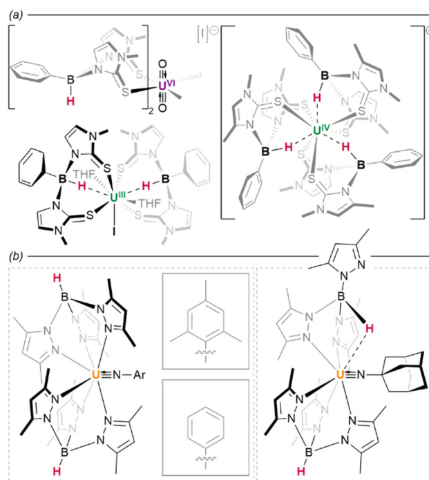
Fig. 23 Borohydride complexes of actinides. (a) With bis(pyrazolyl)borane and bis(methimazolyl)boranes coordination of the B–H bond to the actinide centre is facile. (b) With tris(pyrazolyl)boranes the flexibility in coordination mode may allow for formation of complexes with more sterically encumbered co-ligands.
