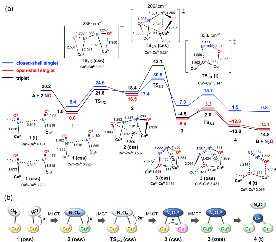
Fig. 6 (a) Free-energy profile for the reduction of NO to N_2O by dicopper complex A. Free energies are expressed in kcal mol -1 . Energies and optimized geometries were calculated at the B3LYP-D3/D95** (Wachters-Hay for Cu) level of theory with the solvent effect of tetrahydrofuran using the polarizable continuum model. (b) Schematic representation of the changes in electronic states during the NO reduction by the dicopper complex. Reproduced from ref. 52 with permission from the Royal Society of Chemistry, copyright 2022.
