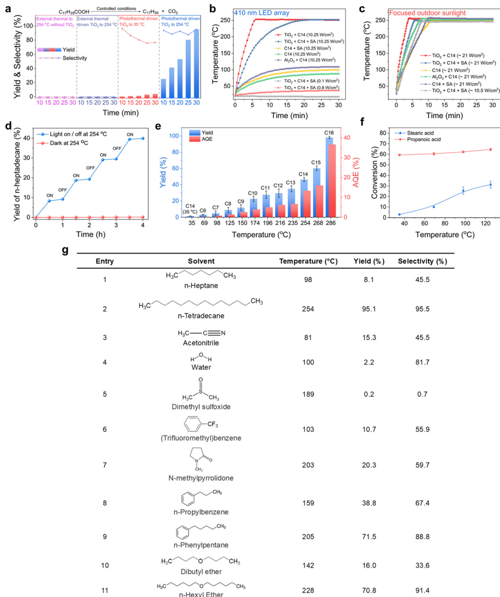
Fig. 2 Photocatalytic decarboxylation of stearic acid over TiO 2 at solvent-locked boiling temperature. (a) Comparison of the yield and selectivity for the decarboxylation of stearic acid under different conditions. (b) Temperature increment for different reaction media under the same LED light irradiation and (c) under focused outdoor sunlight. (d) Alternating on and off light experiments for the decarboxylation of stearic acid at solvent-locked temperature ( n -tetradecane, 254 °C) and full-course dark reaction at 254 °C maintained by an external heat source without light irradiation. (e) Yields and AQEs for the photocatalytic decarboxylation of stearic acid at different boiling points with a range of n -alkanes acting as the solvent. (f) Promotion difference by the self-heating effect between stearic acid and propanoic acids (from 35 °C to 125 °C). (g) TiO 2 -based photothermal catalytic decarboxylation of stearic acid in some solvents with different polarities and boiling points. General reaction conditions: reaction solution volume (25 mL), TiO 2 (125 mg), stearic acid (0.05 M), n -octadecane (internal standard, 0.05 M), reaction pressure (0.1 MPa), solvents locked reaction temperature, N 2 atmosphere, LED (410 nm, 10.25 W cm -2 ) irradiation for 15 min in (e) and for 30 min in (g). All the catalytic performance data in the figures are averages of at least three experiments.
