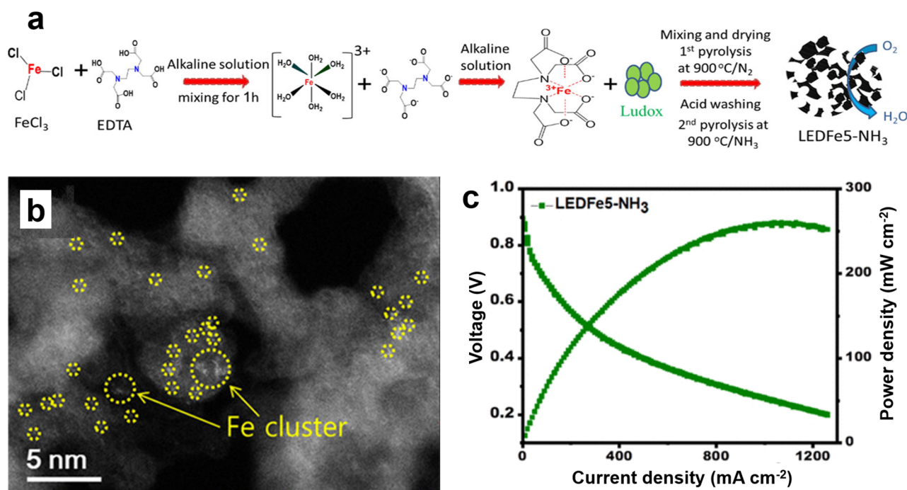
Fig. 12 (a) Schematic illustration of synthesis process for EDTA–Fe complex-based catalyst; (b) HAADF-STEM image of \text{LEDFe}_5\text{-NH}_3 ; (c) single-cell performance of HT-PEMFC at 1.5 \text{ bar O}_2 pressure and 150^\circ\text{C} cell temperature. Reprinted with permission from ref. 62. Copyright 2014, American Chemical Society.
